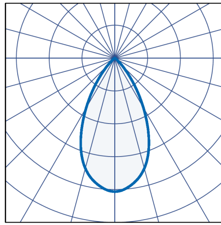
60° Optic:
