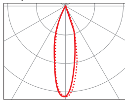
15° Optic
